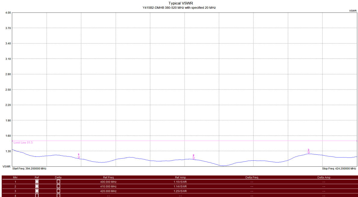
Typical VSWR at a specified 20 MHz bandwidth
