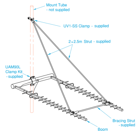
Y415B2-DMBH with included strut kits + UV1-SS and UAM90L fitted to reduce mechanical downtilt and movement
